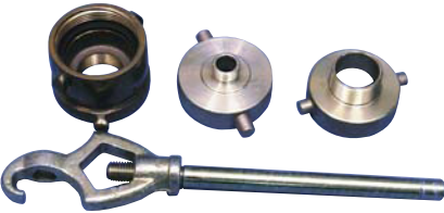
Adjustable Hydrant Wrench #AHW
